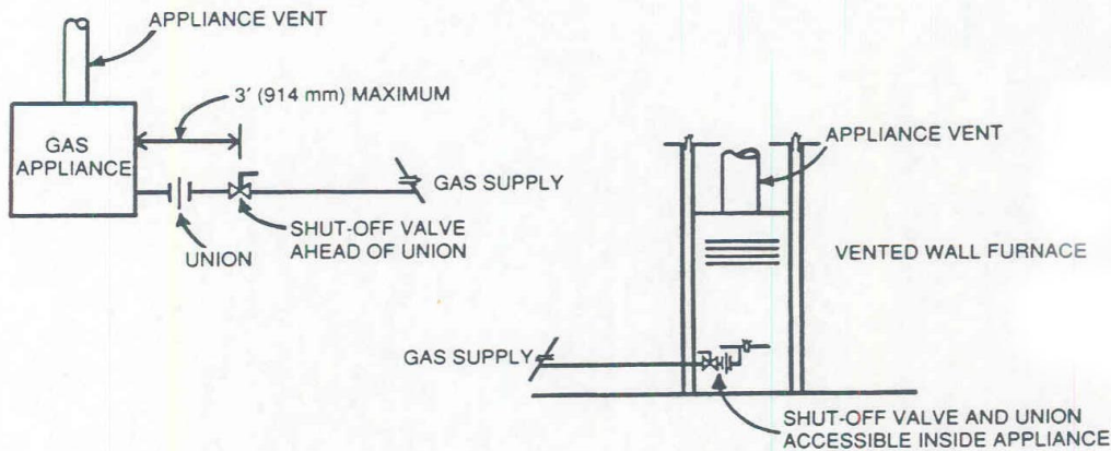
RIGID GAS CONNECTIONS, THREADED PIPE AND FITTINGS
