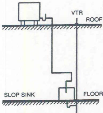
F—ACCEPTABLE WITH STRAINER ONLY. NO PLUG OR STOPPER
