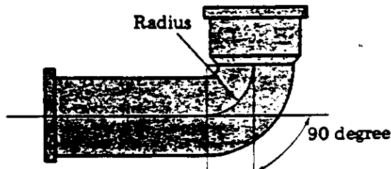
Low-hub 1/4 bend, also used to receive the waste from water closets, by caulking a lead stub into hub
