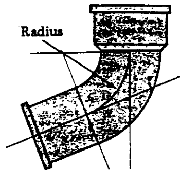
1/5 bend 72 degree illustrated 1/6 bend 60 degree
