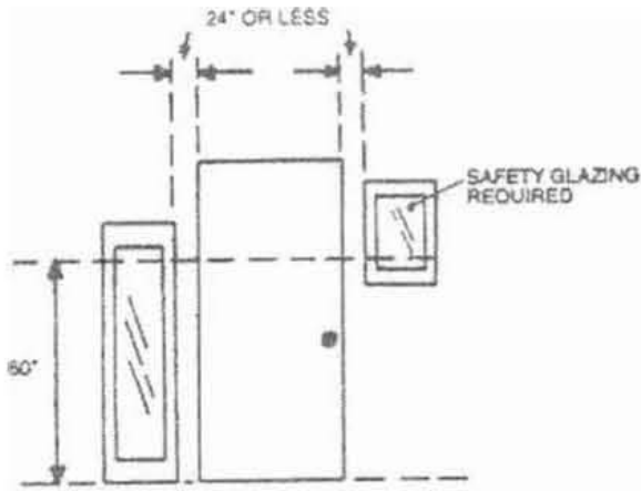
GLASS IN SIDELIGHTS—ELEVATION
