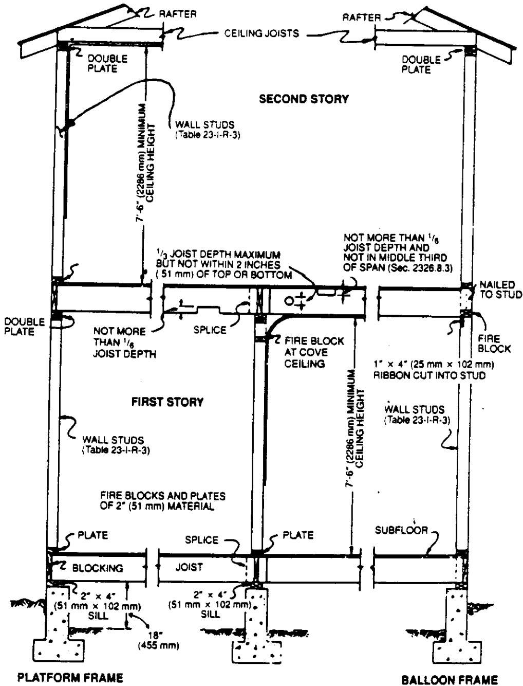
FIGURE 6—FRAMING SECTION
