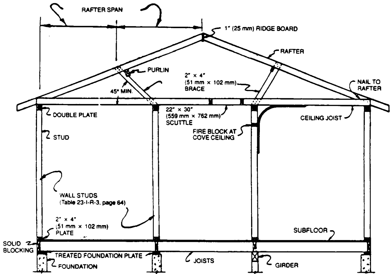
FIGURE 9—ROOF FRAMING DETAIL
