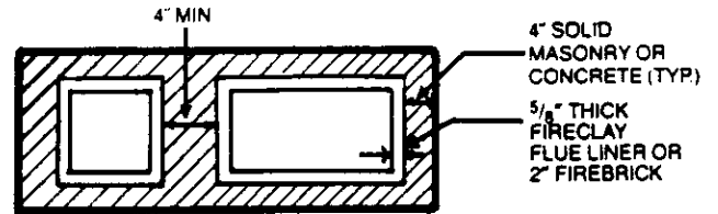
LINED MULTIPLE-FLUE CHIMNEY
