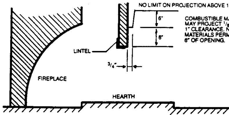
COMBUSTIBLE MATERIALS PROJECTION FROM FIREPLACE
