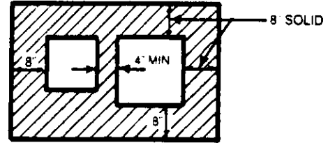
REQUIRED PROTECTION AROUND UNLINED FLUES
