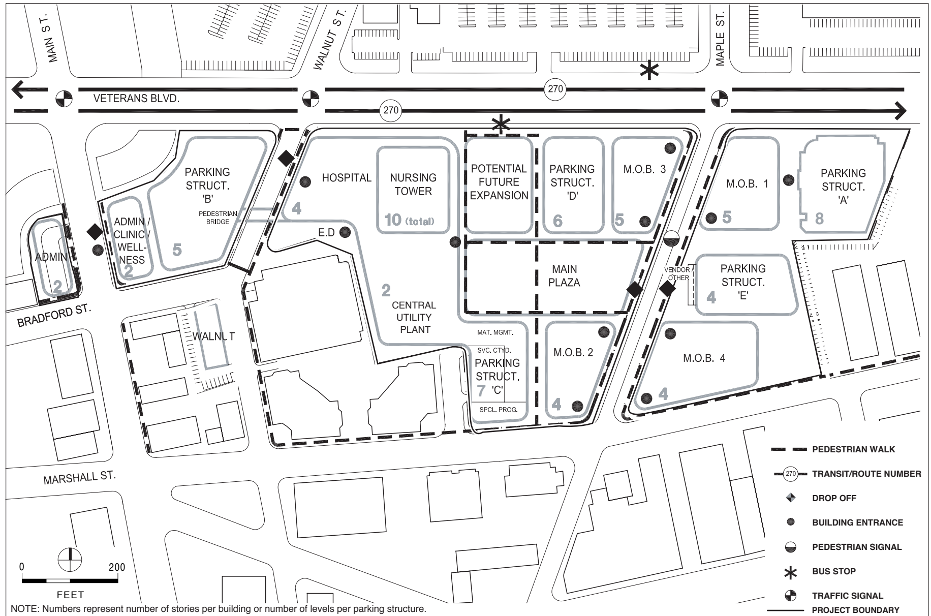
KAISER REDWOOD CITY MASTER PLAN EIR FIGURE 2-6: PEDESTRIAN CIRCULATION PLAN
