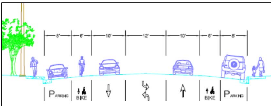
Proposed lane configuration (typical)
