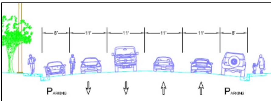
Existing lane configuration
