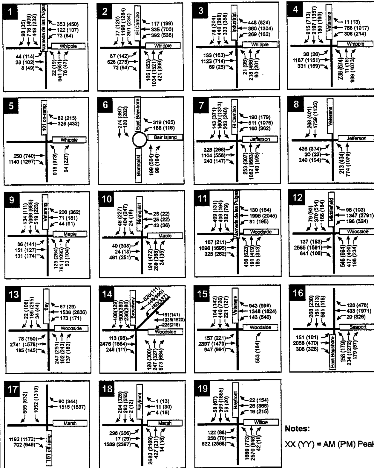
Figure 7.10 CUMULATIVE (2020) WITHOUT PROJECT PEAK-HOUR INTERSECTION VOLUMES
