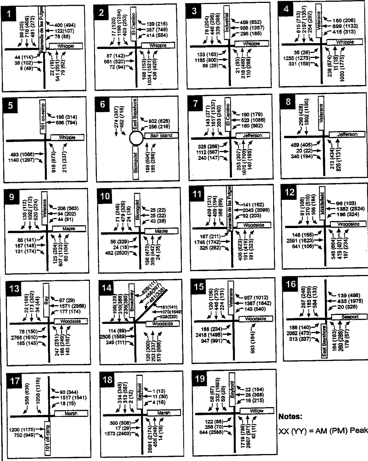
Figure 7.11 CUMULATIVE (2020) WITH PROJECT PEAK-HOUR INTERSECTION VOLUMES
