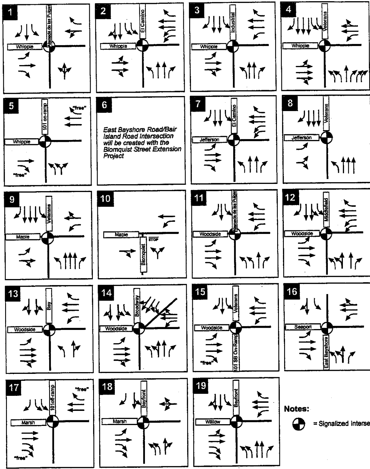
Figure 7.2 EXISTING INTERSECTION LANE CONFIGURATIONS
