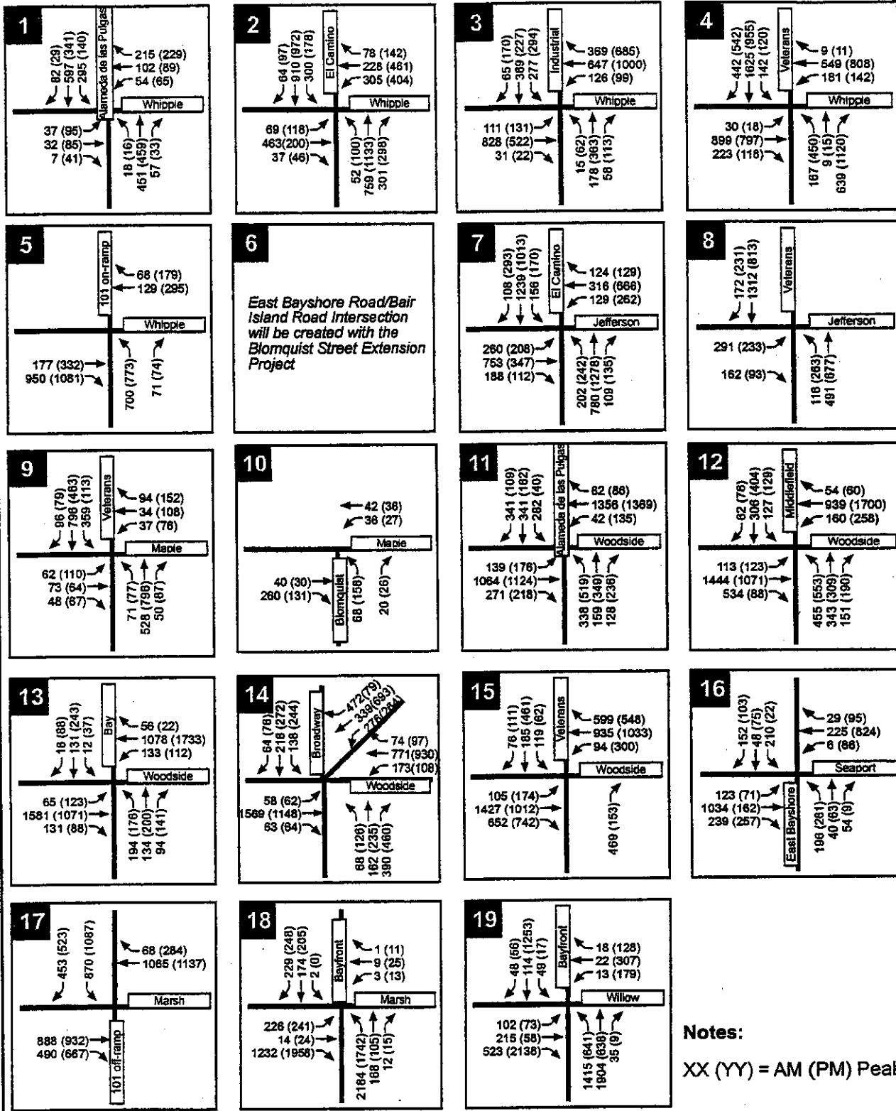
Figure 7.3 EXISTING PEAK-HOUR INTERSECTION VOLUMES
