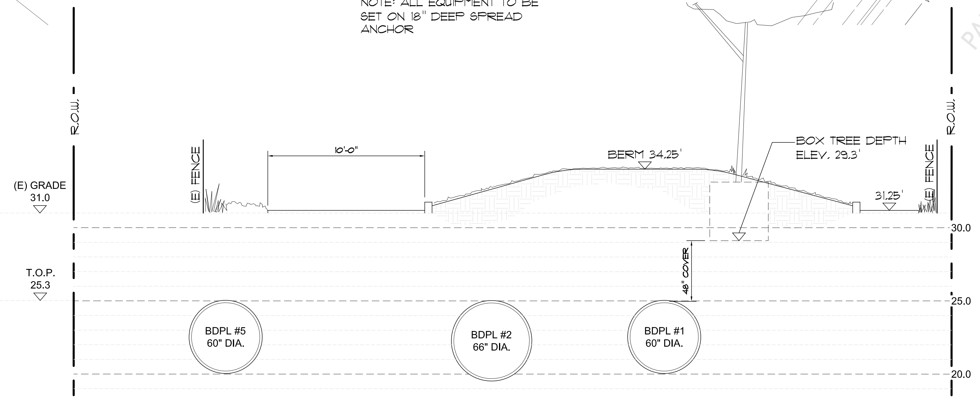
A SECTION AT LANDSCAPE BERM SCALE: 1/4" = 1'-0"
