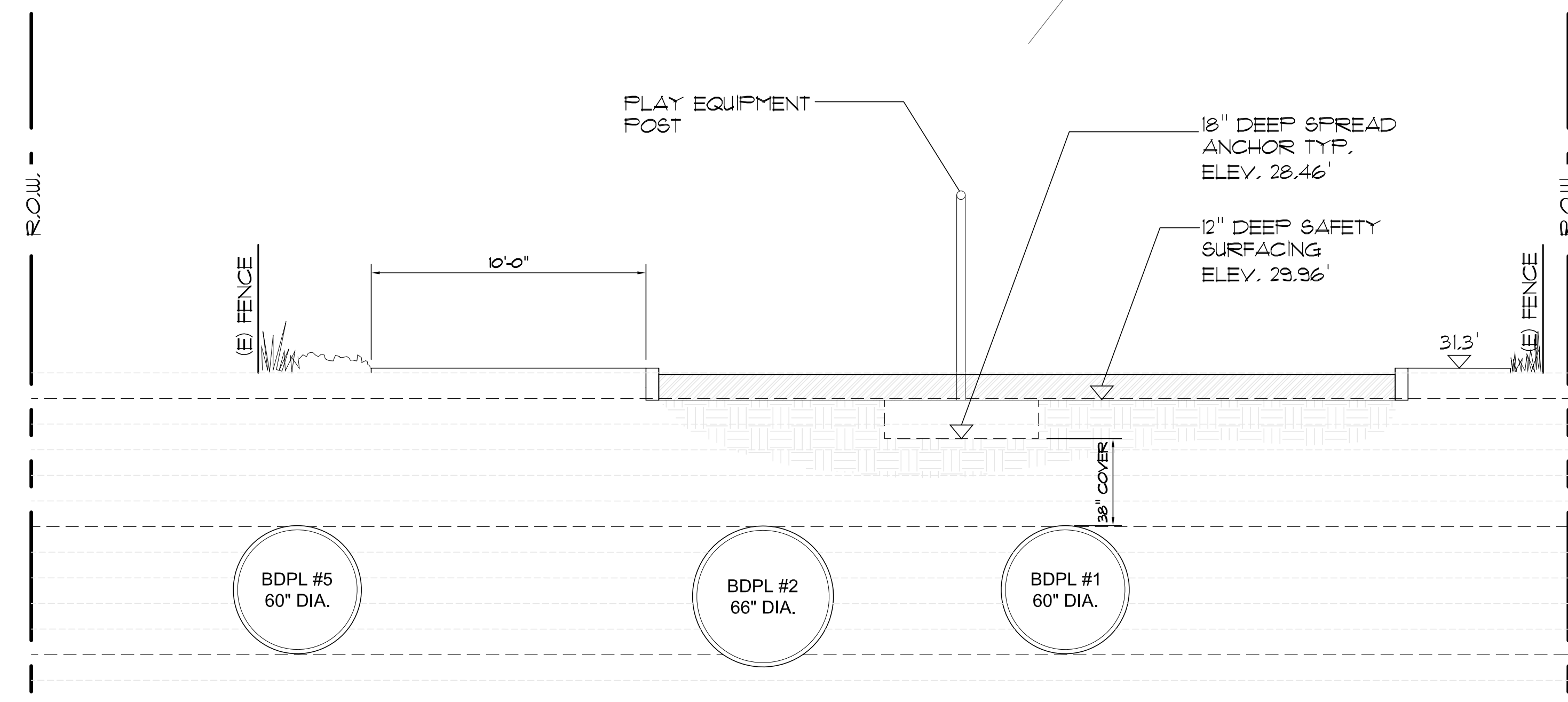
B SECTION AT PLAY EQUIPMENT SCALE: 1/4" = 1'-0"
